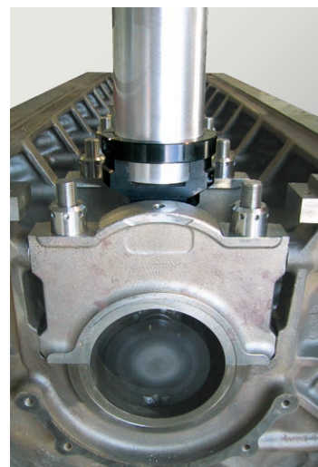
Special steel main bearing housings found in high power diesel engines such as MTU 4000 require high speed machining to obtain superior accuracy of roundness, straightness, parallelism and surface finish.
